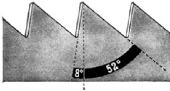
Side view of rip teeth (enlarged)
